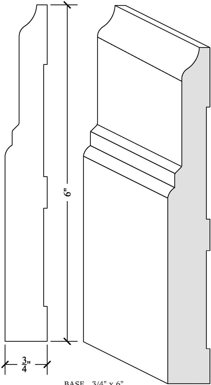
BASE 3/4" x 6" BAS-131
