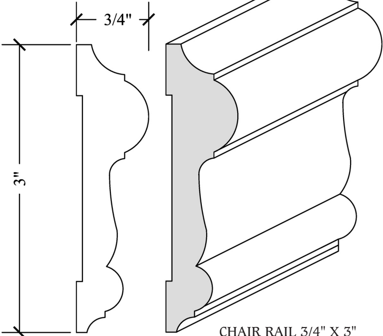
CHAIR RAIL 3/4" X 3" CHR-140
