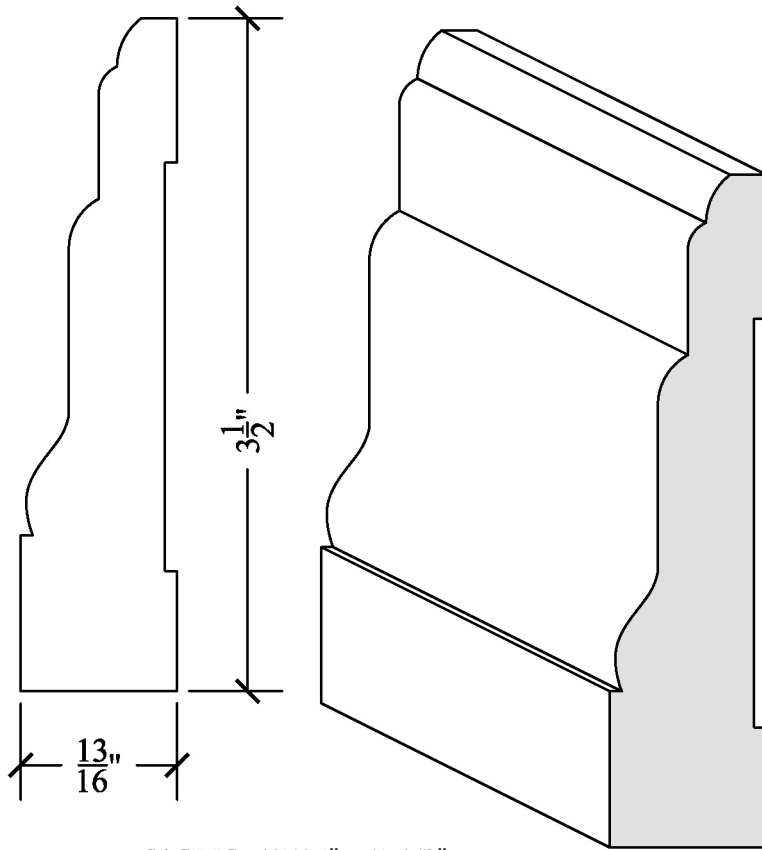
CASING \frac{13}{16} " x 3\frac{1}{2} " CAS-130
