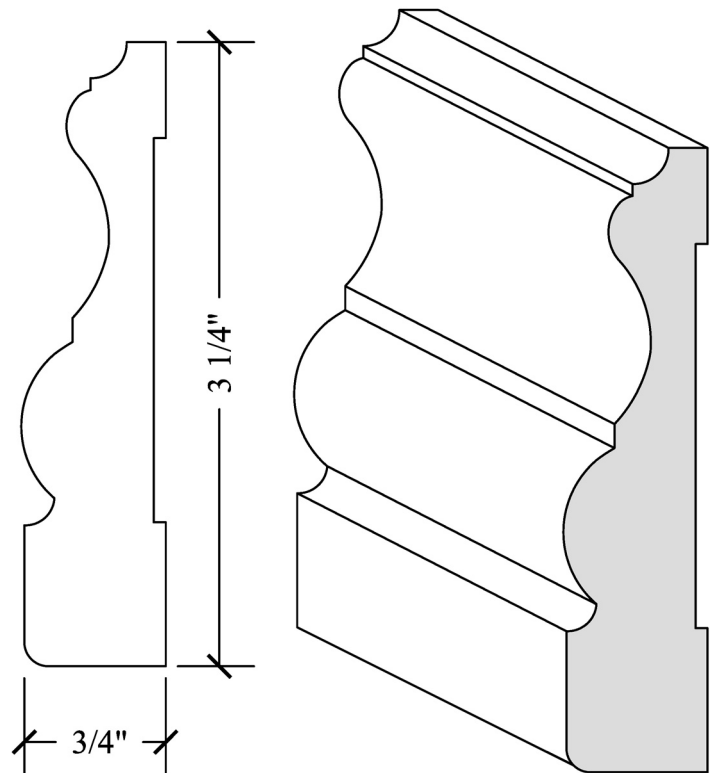
CASING \frac{3}{4} " x 3\frac{1}{4} " CAS-132
