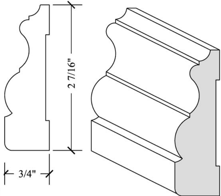
CASING 3/4" x 2-7/16"
