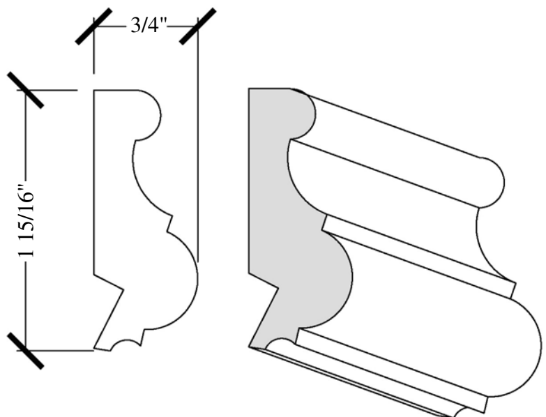
PANEL MOLD/BASE CAP 3/4" x 1-15/16"
