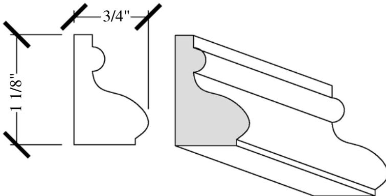
PANEL MOLD/BASE CAP 3/4" x 1-1/8"
