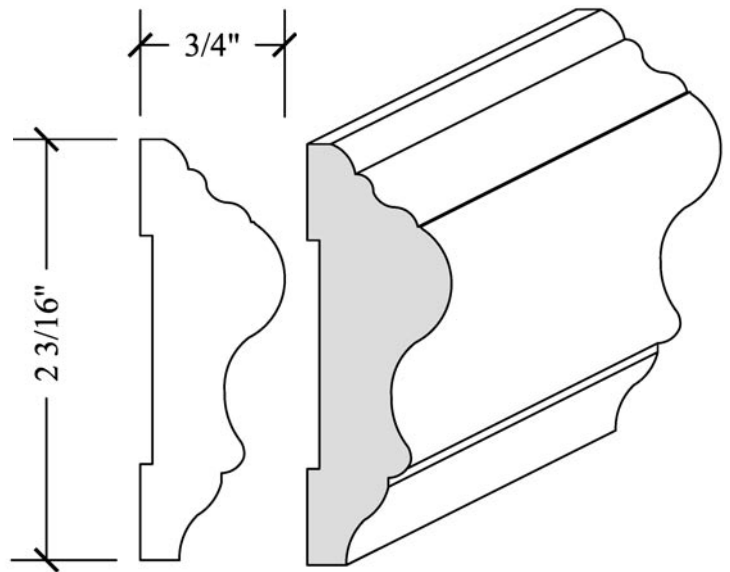
CHAIR RAIL 3/4" X 2-3/16"
