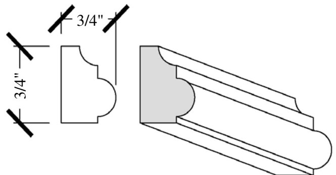
PANEL MOLD/BASE CAP 3/4" x 3/4"
