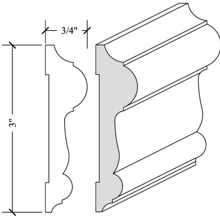
CHAIR RAIL 3/4" X 3"
