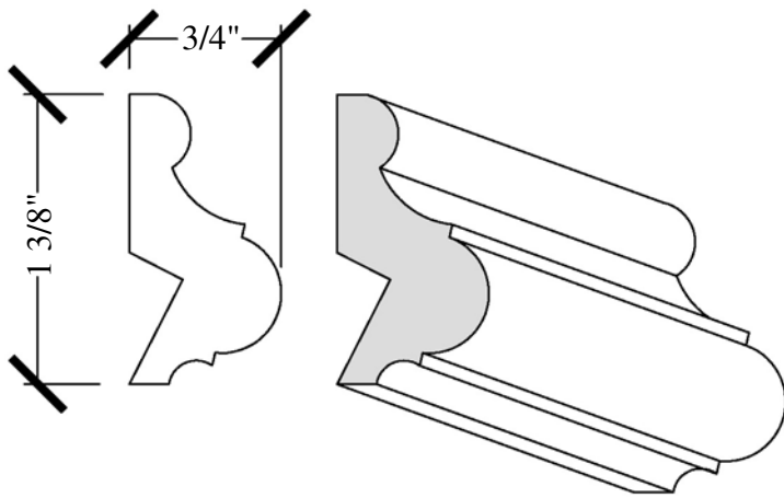
PANEL MOLD/BASE CAP 3/4" x 1-3/8"
