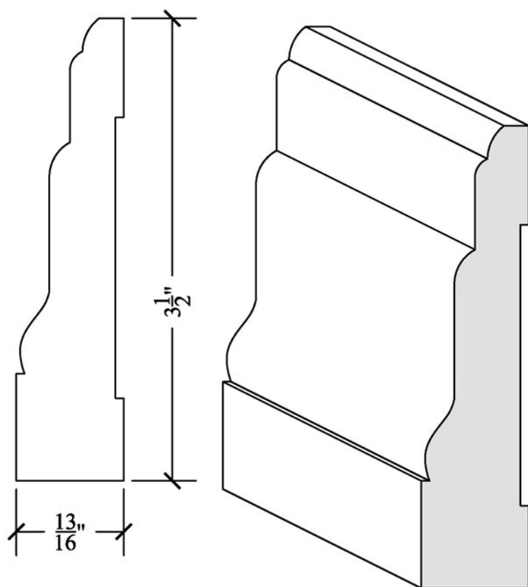
CASING 13/16" x 3-1/2"
