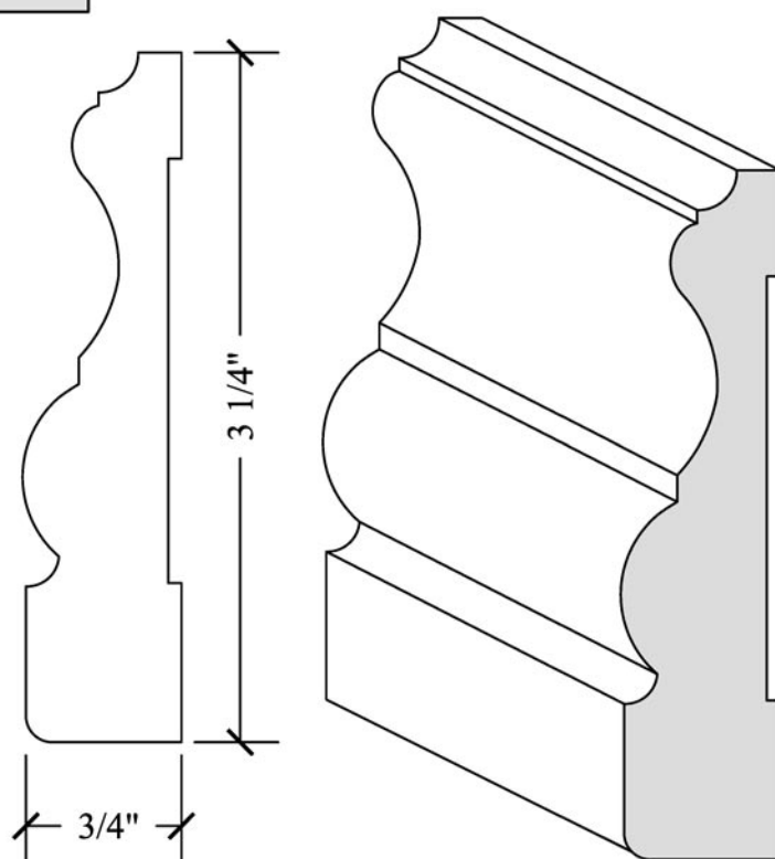
CASING 3/4" x 3-1/4"
