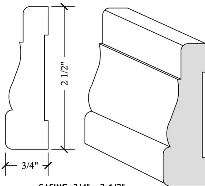
CASING 3/4" x 2-1/2"
